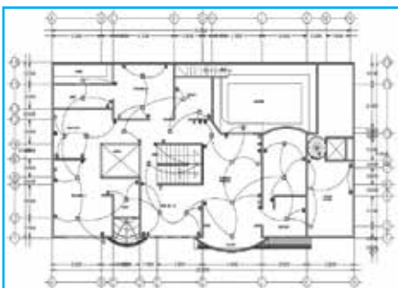
Electrical Layout Design
